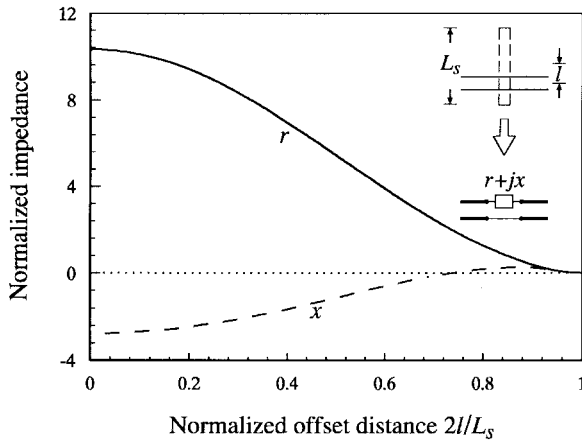
Fig. 2. Normalized equivalent series impedance of a slot antenna fed by an infinitely long microstrip line, as functions of the normalized offset distance ( 2l/L_s ). f = 3.02 GHz.
